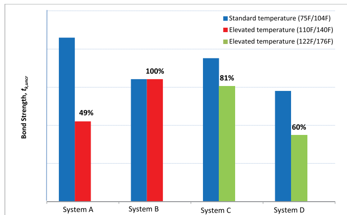
Figure 3: Comparison of the Characteristic Bond Strength for Various Adhesive Products
